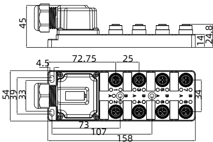
Eight-hole junction box without cable
