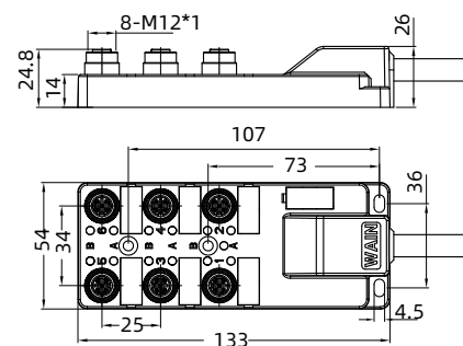
• Six-hole double channel junction box with cable
