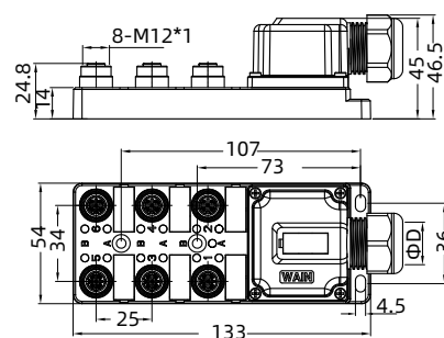
• Six-hole double channel junction box without cable
