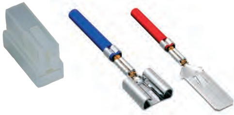
Receptacles, insulation sleeves and housing
