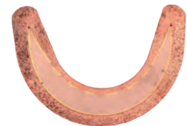
Deep Indent on Aluminum Flexible Cable
