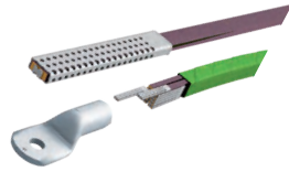
Embedded transformer terminals
