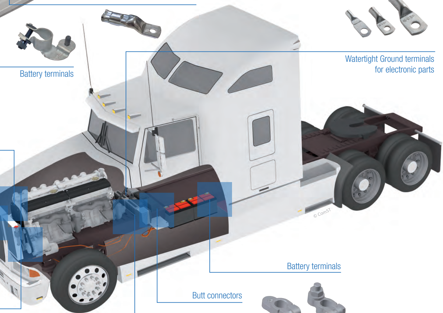
DBI terminals for Aluminum cables
