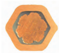
Watertight Crimp on Cable Insulation
