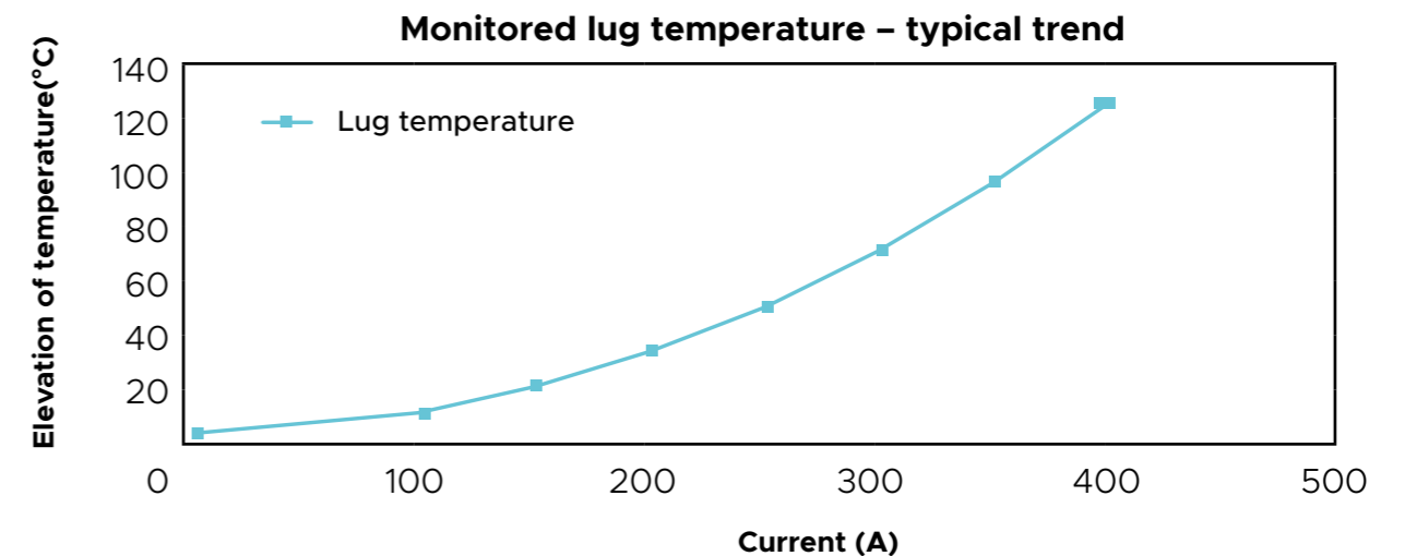
Lug temperature elevation under injected current
