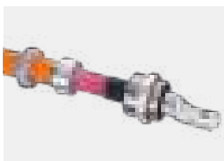
1. Kabelschuh durchschieben 1. Push cable lug through
